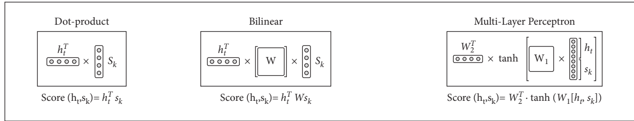
FIGURE 9: Calculation of attention scores.
