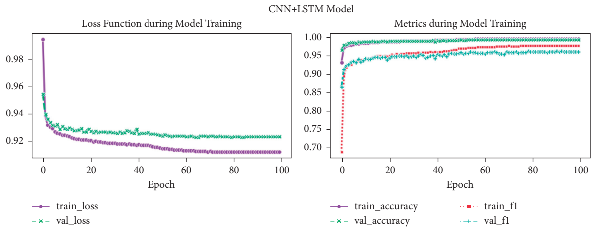
FIGURE 12: CNN and LSTM model.
