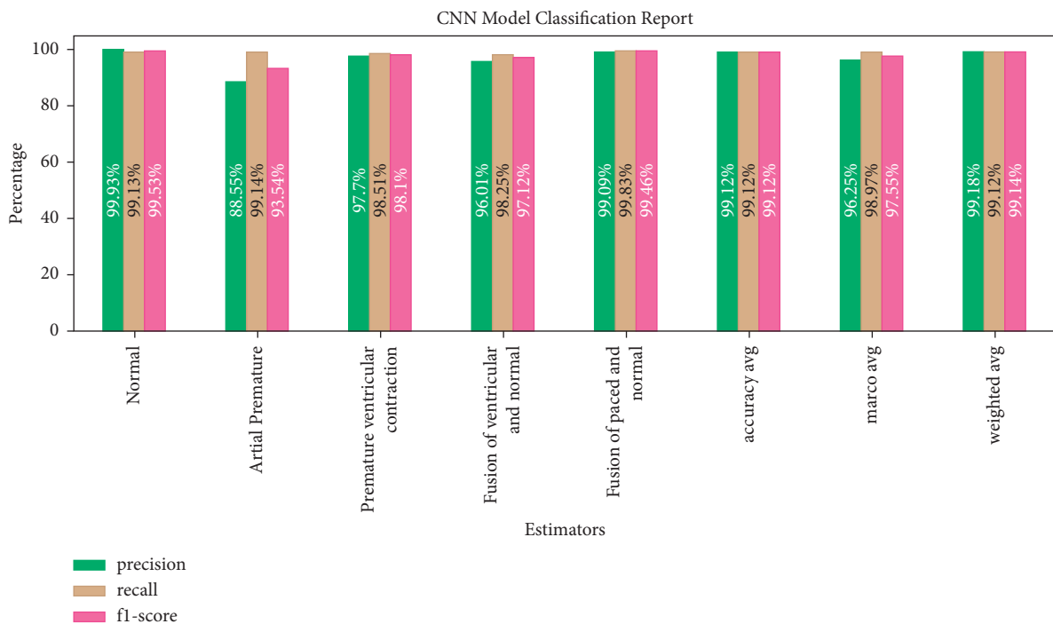
FIGURE 14: CNN model classification report.
