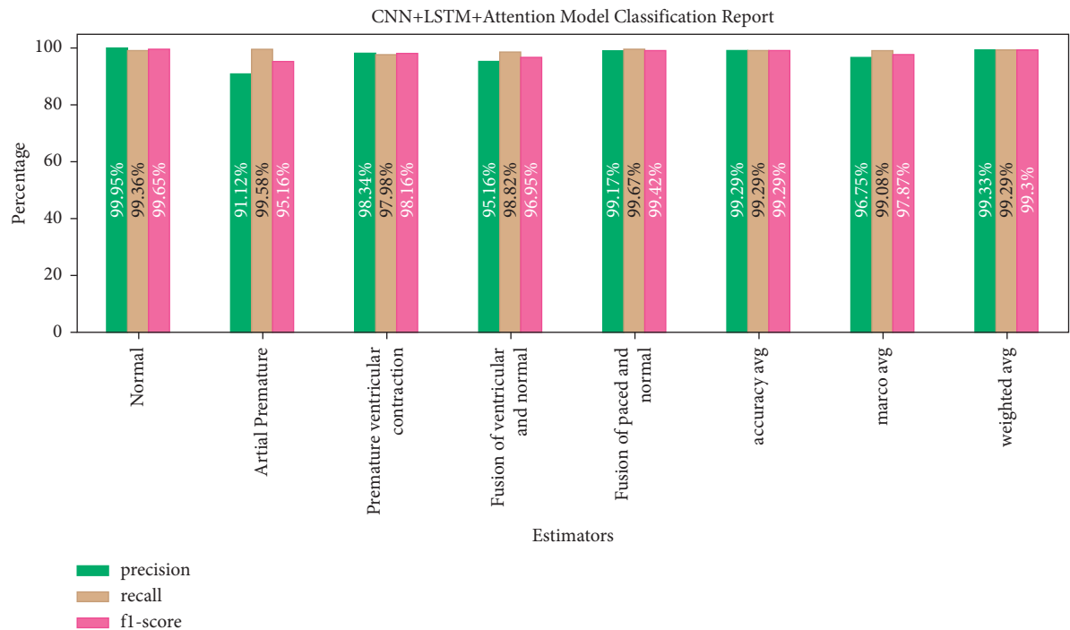
FIGURE 16: CNN + LSTM + Attention Model classification report.
