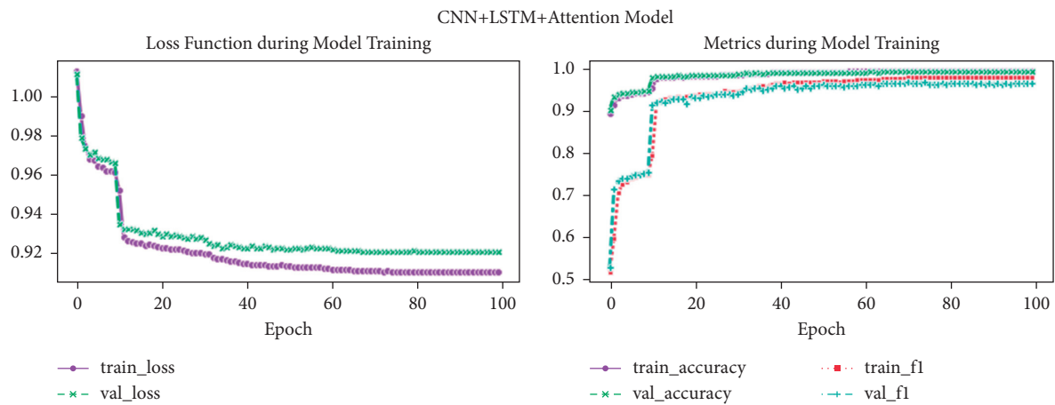
FIGURE 13: CNN + LSTM + Attention Model.
