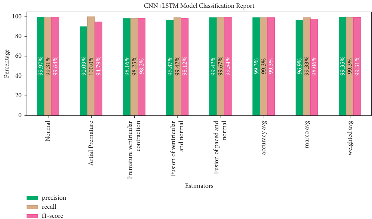
FIGURE 15: CNN + LSTM model classification report.
