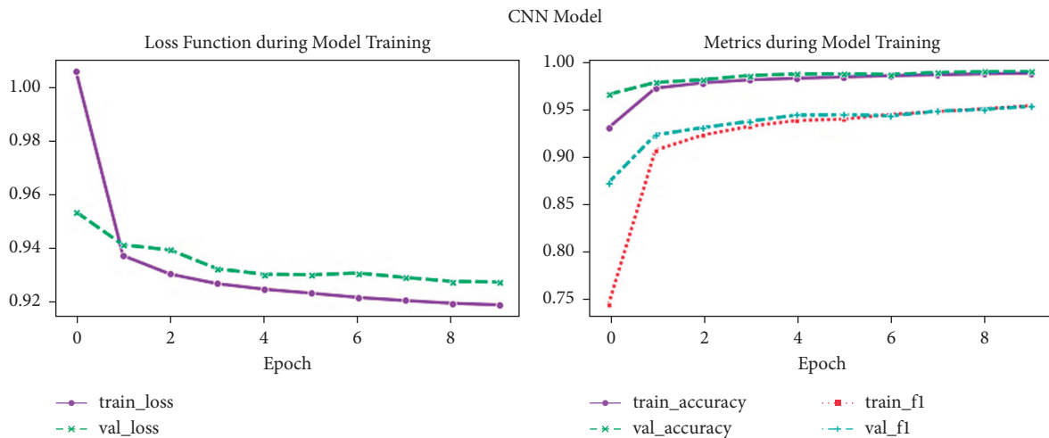
FIGURE 11: CNN model performance.
